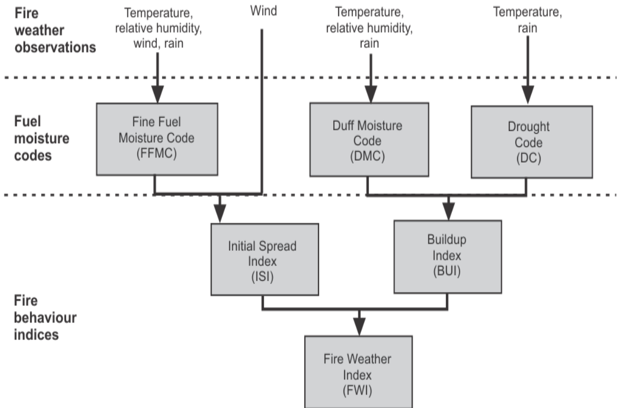
Figure 2. Structure of the Canadian Forest Fire Weather Index System (FWI system) (from http://cwfis.cfs.nrcan.gc.ca/en/background/bi_FWI_summary_e.php ).
